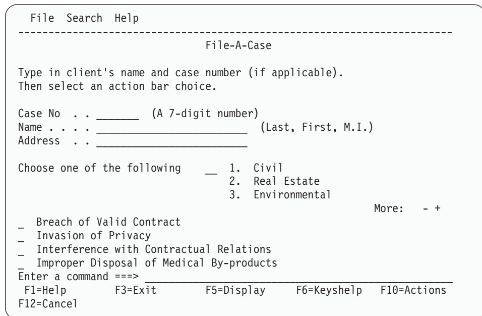
Figure 16. Application panel area
