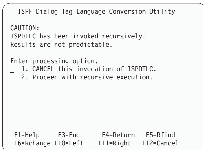
Figure 85. ISPF Dialog Tag Language conversion utility - recursive invoke
