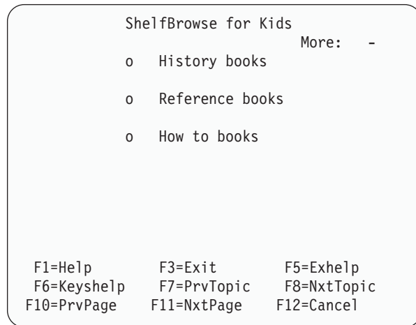
Figure 123. Help panel (example 3 of 3)
