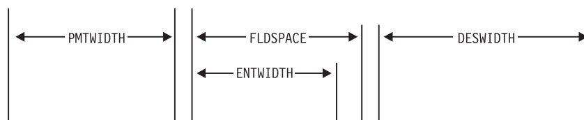
Figure 109. PMTWIDTH, ENTWIDTH, FLDSpace, and DESWIDTH attributes
