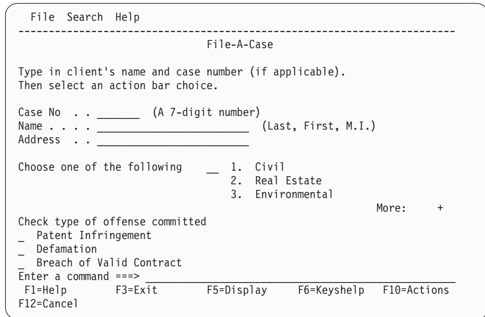
Figure 15. Scrollable panel area
