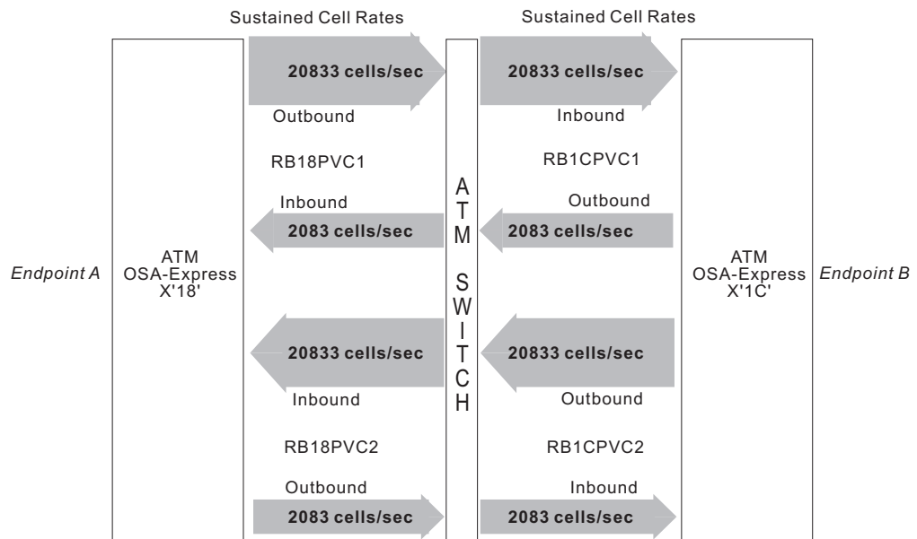
Figure 71. Two Virtual Circuits with One Inbound and One Outbound
