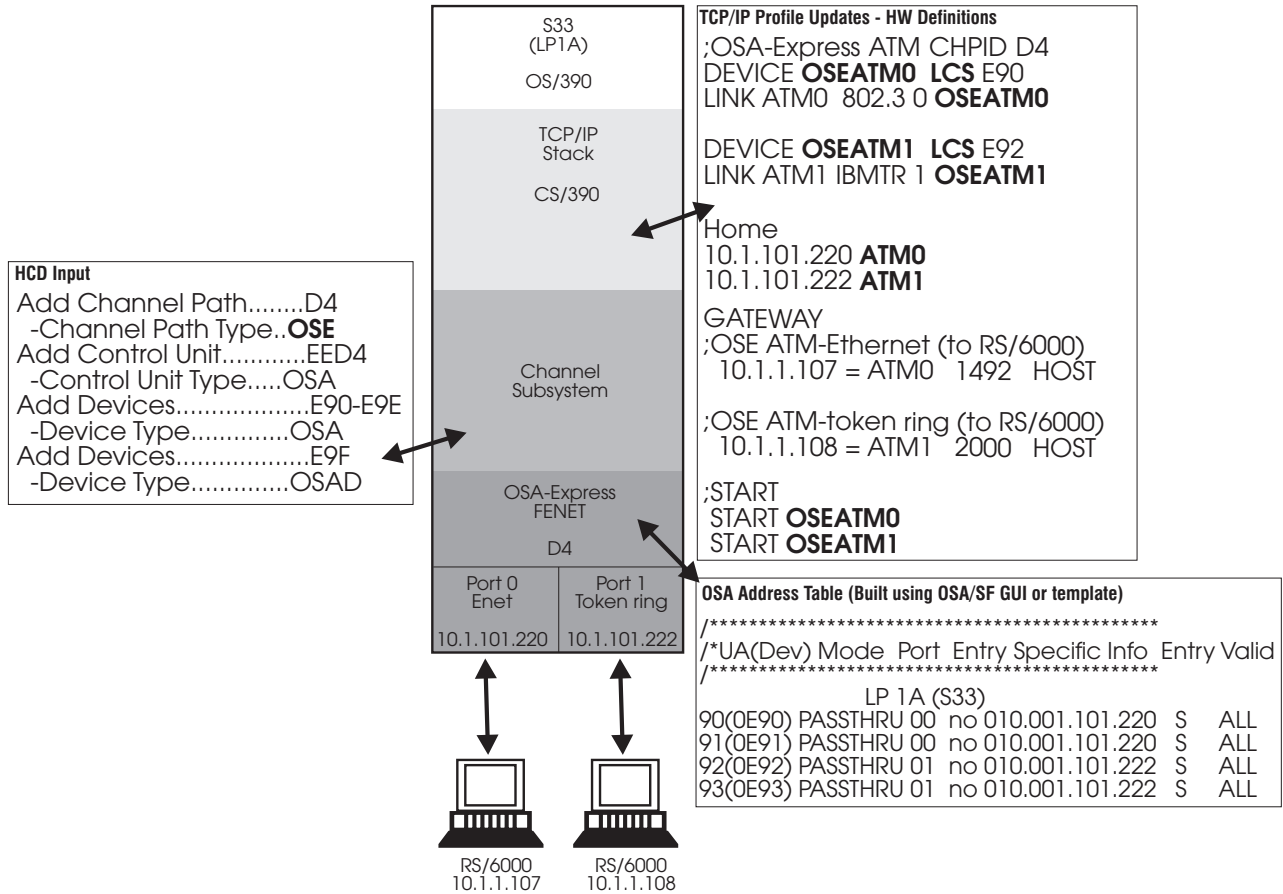
Figure 110. Ethernet and Token Ring Passthru on ATM LANE
