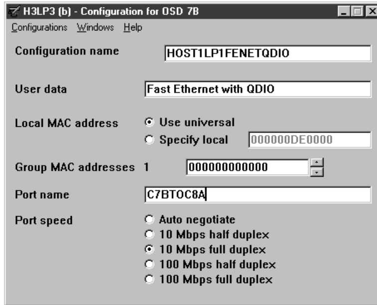
Figure 76. FENET Configuration for OSD Channel
