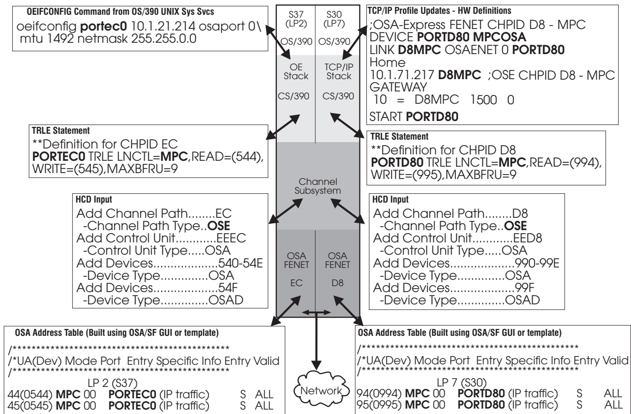
Figure 115. HPDT MPC on OSA-Express FENET. The netmask of 255.255.0.0 is unique and specific to our test environment. You will need to use the subnet mask appropriate to your environment.
