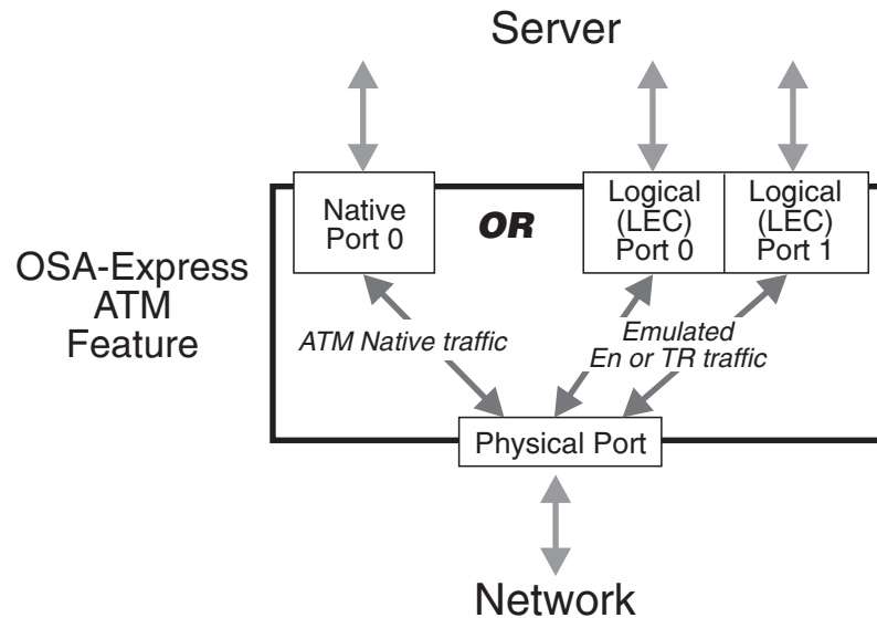
Figure 4. The OSA-Express ATM Feature Supports One Port for ATM Native and Two Emulated Ports for LEC Services
