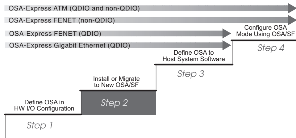
Figure 31. Step Two (VM) in a Four-Step Process
