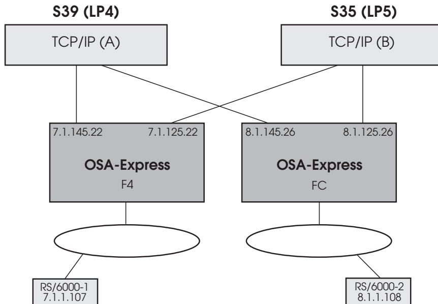
Figure 105. Test Configuration 1 – No Primary/Secondary Routing
