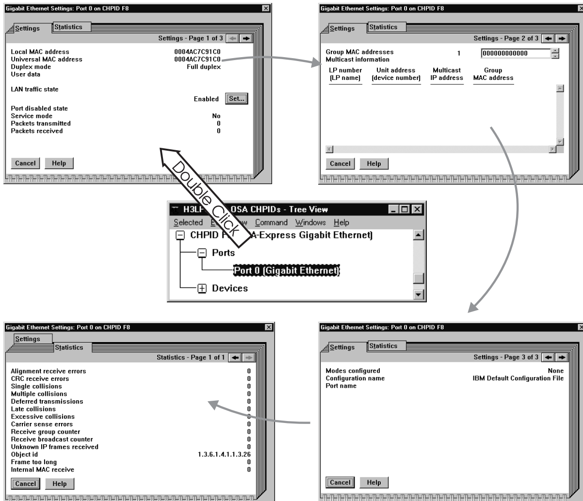
Figure 86. OSA-Express Gigabit Ethernet Settings
