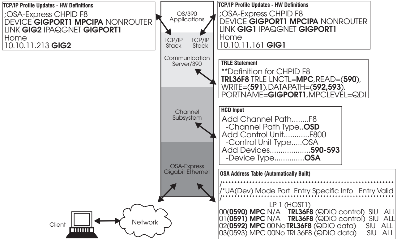
Figure 117. OSA-Express GbE Definitions for S/390 with Two TCP/IP Stacks
