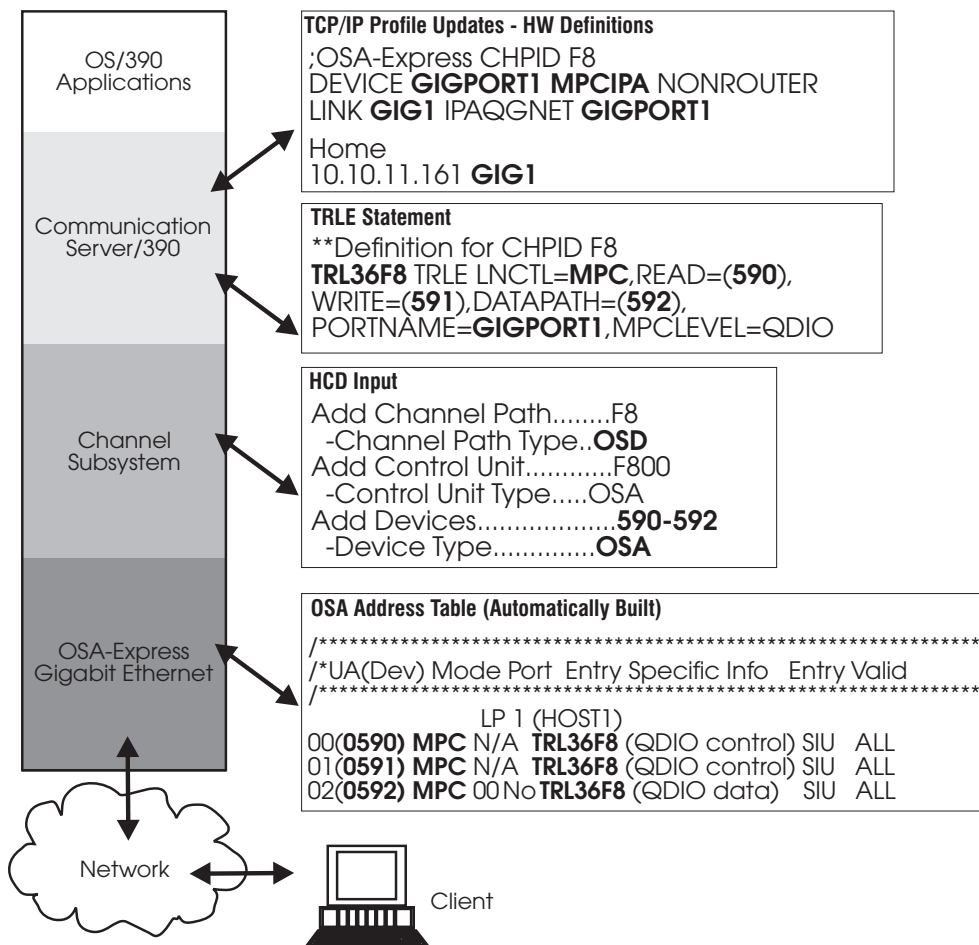
Figure 116. OSA-Express GbE Definitions for S/390 in BASIC Mode — No Logical Partitions
