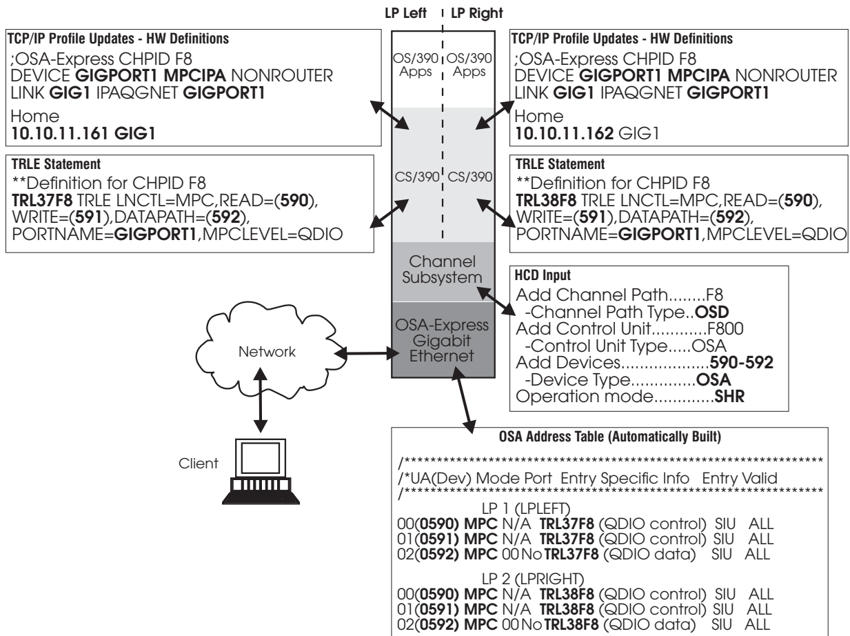
Figure 118. OSA-Express GbE Definitions for S/390 in LPAR Mode with Two Logical Partitions
