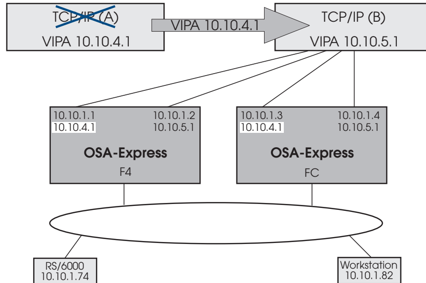
Figure 9. DVIPA Automatically Relocates When TCP/IP Stack Fails
