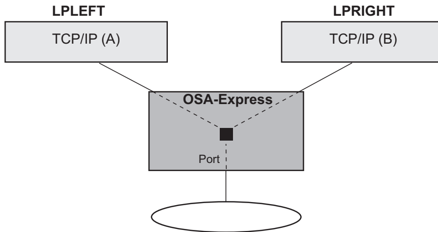
Figure 6. Port Sharing Allows Multiple Partitions Access to OSA-Express Ports
