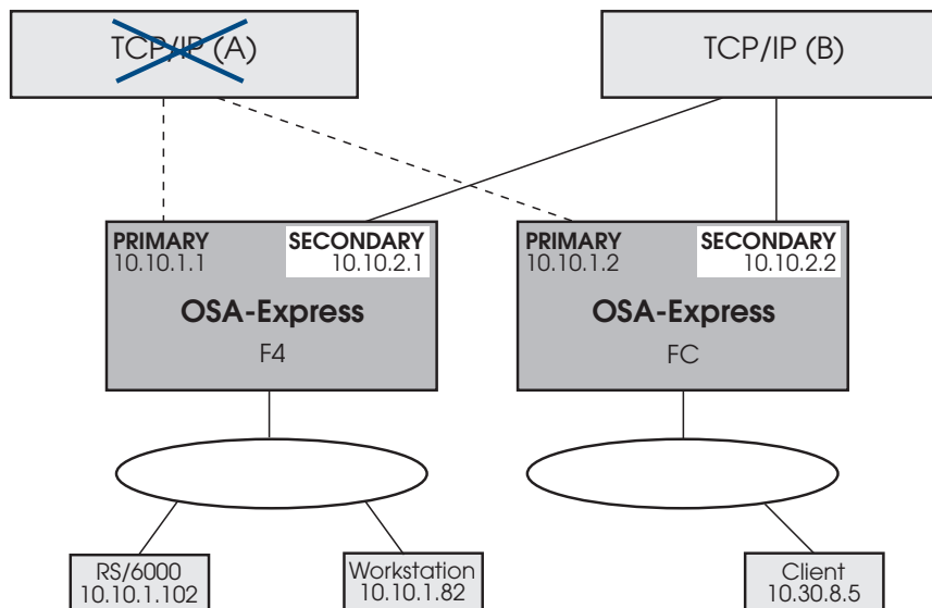
Figure 8. Secondary Router Provides Path to Unknown IP Addresses When Primary Router Fails
