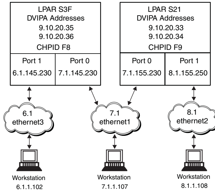
Figure 113. Two OSA-Express ATM Features Configured for Ethernet LAN Emulation with Dynamic VIPA
