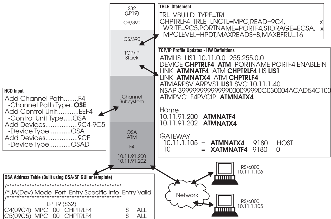
Figure 109. Classical IP over ATM Native
