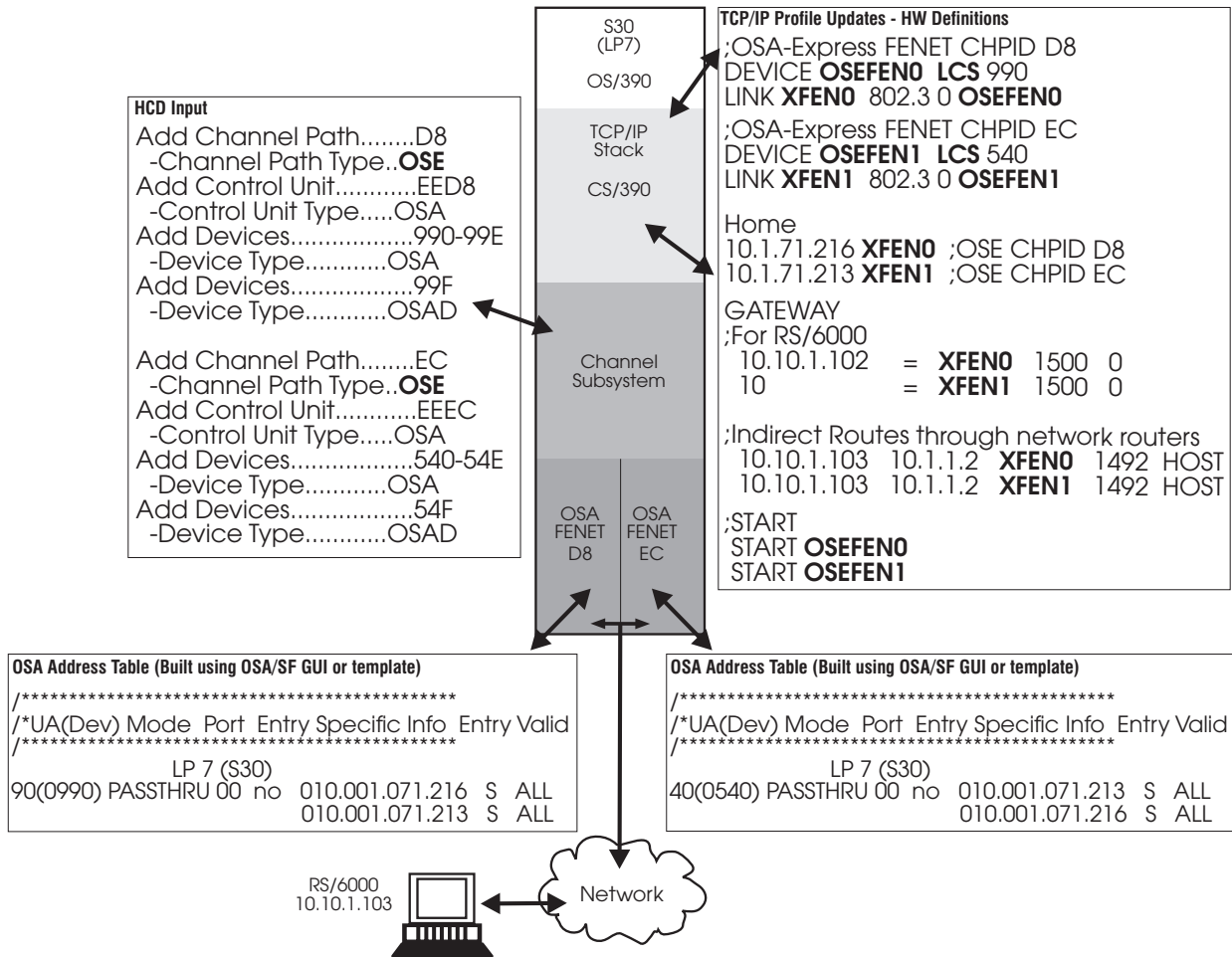
Figure 114. Multiple IP Passthru Entries
