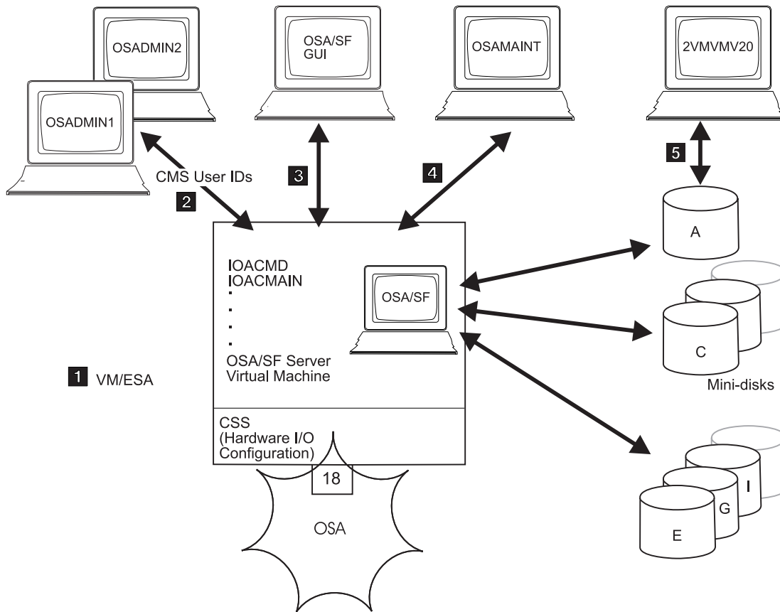
Figure 34. Setup Tasks for OSA/SF in the VM Environment
