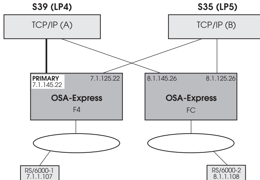
Figure 106. Test Configuration 1 – F4 Primary on S39
