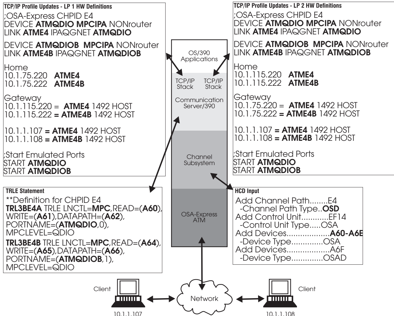
Figure 111. OSA-Express ATM Configured for QDIO on ATM with Two Logical Partitions
