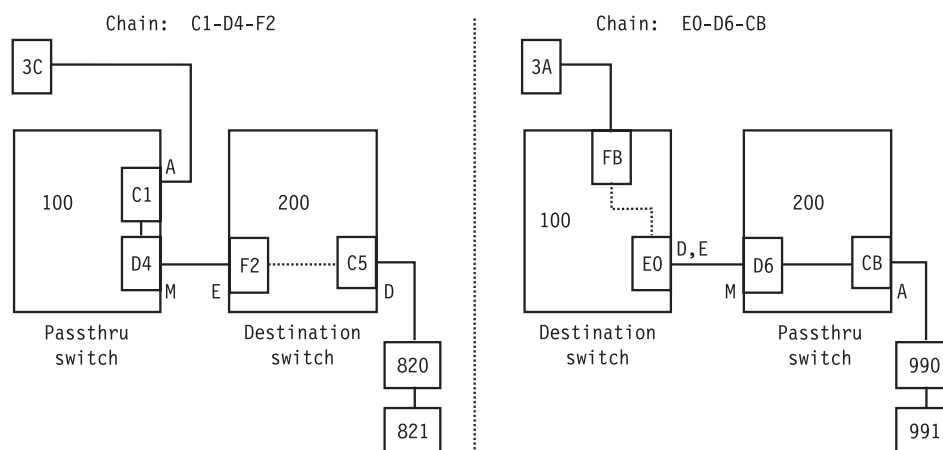
Figure 150. Examples of Chained Paths.
