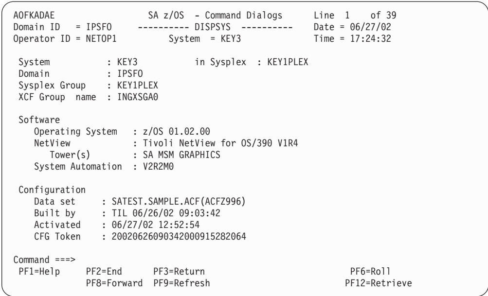
Figure 32. DISPSYS Command Dialog Panel
