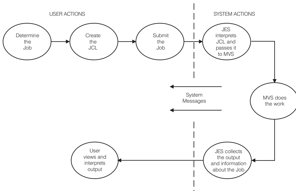
Figure 1. JCL-Related Actions (User and MVS)
