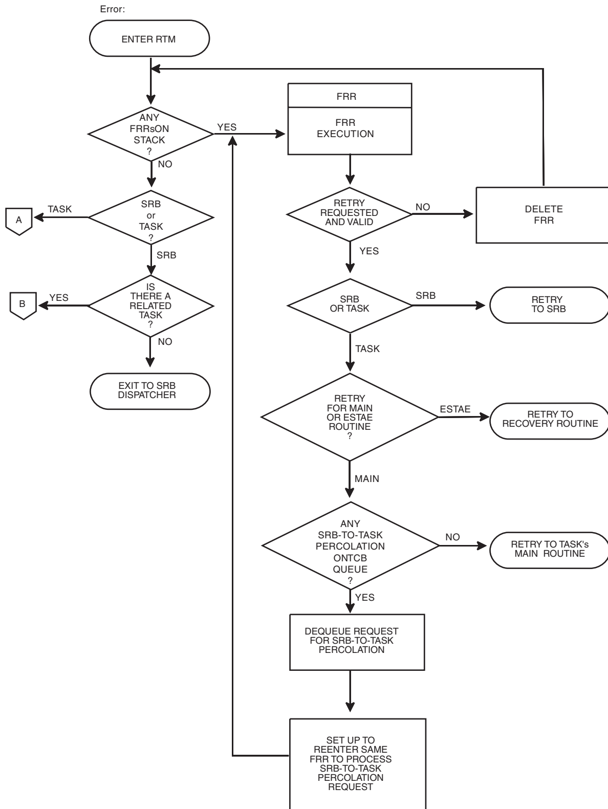
Figure 18-5. Routing Control to Recovery Routines (Part 1 of 3)
