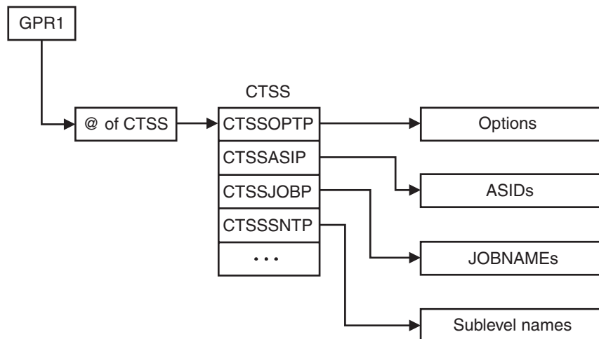
Figure 6-7. Information Passed to the Start/Stop Exit Routine Through GPR 1
