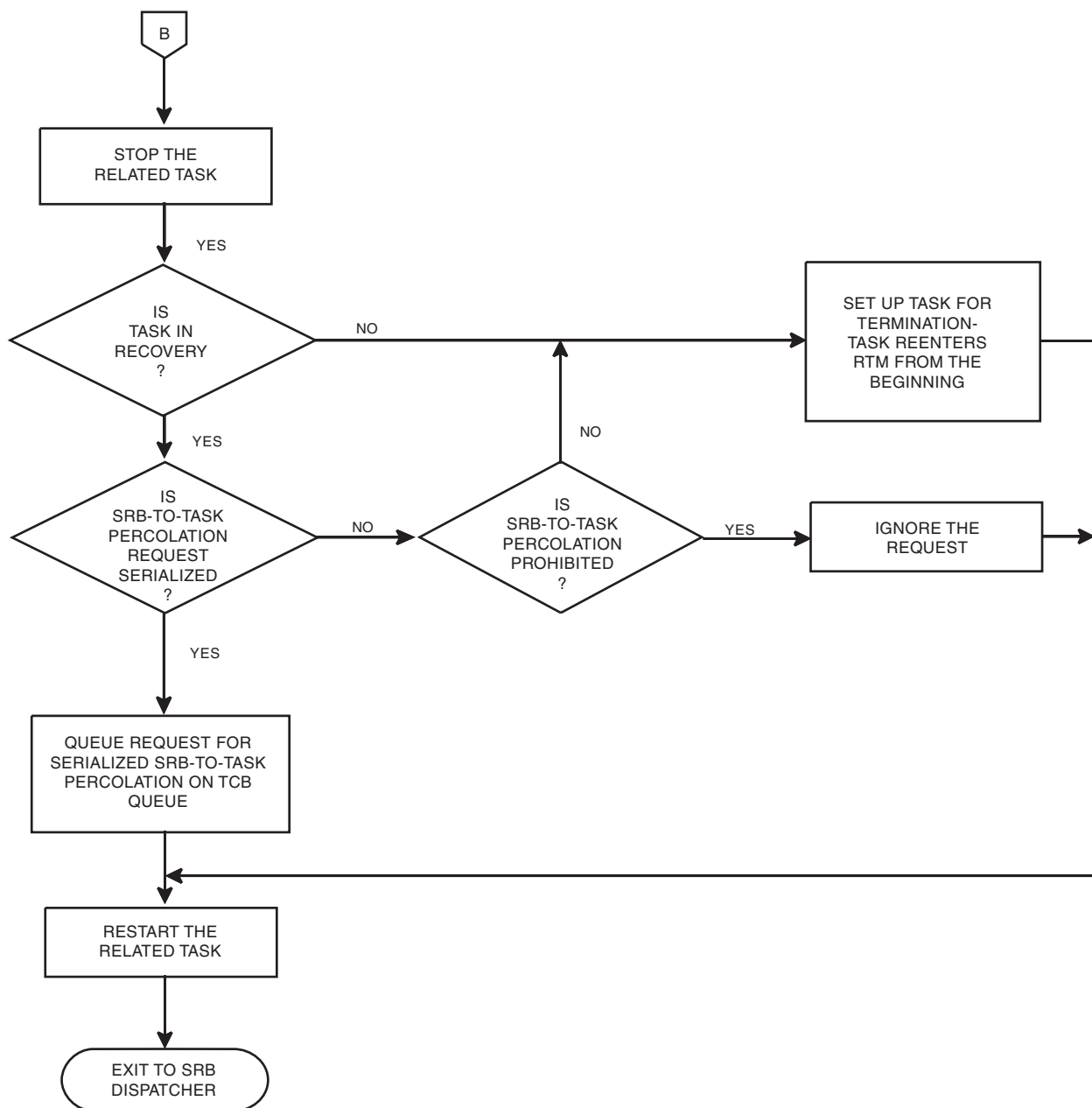
Figure 18-5. Routing Control to Recovery Routines (Part 3 of 3)
