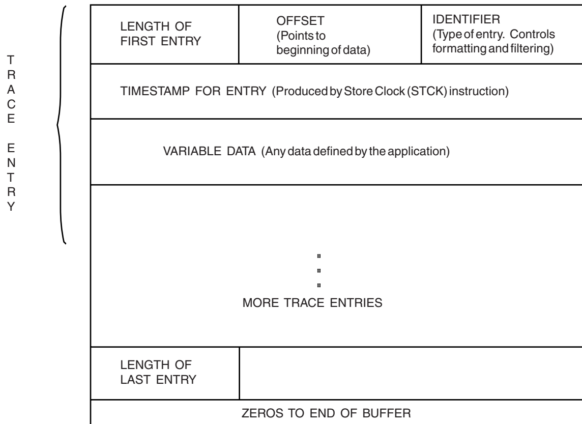
Figure 6-9. Component Trace Entry in a Trace Buffer
