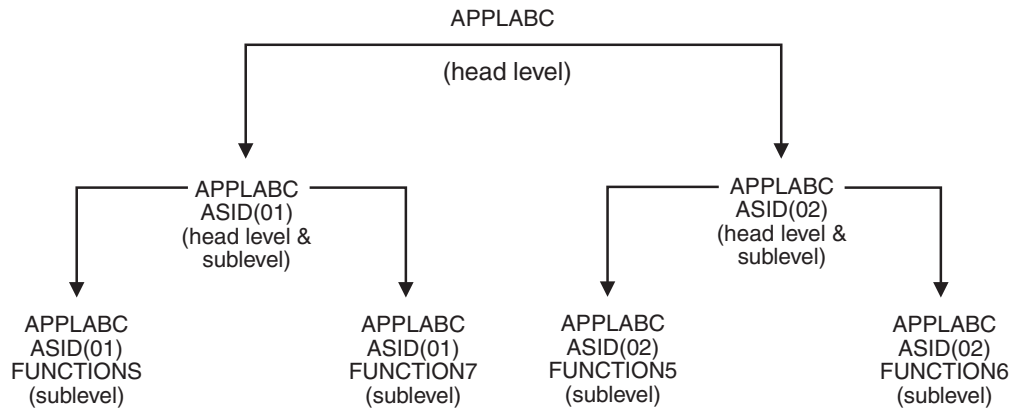
Figure 6-3. Structure of Multiple Traces for an Application
