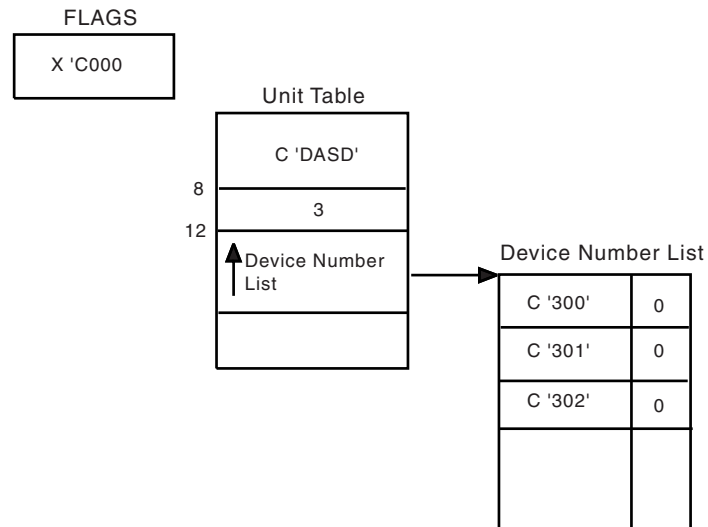
Figure A-19. Input for Function Codes 0 and 1
