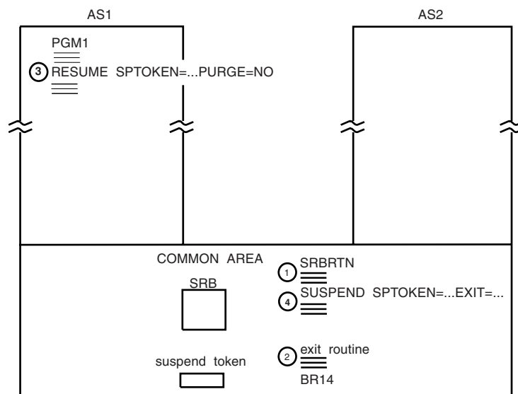
Figure 9-2. Suspending and Resuming an SRB
