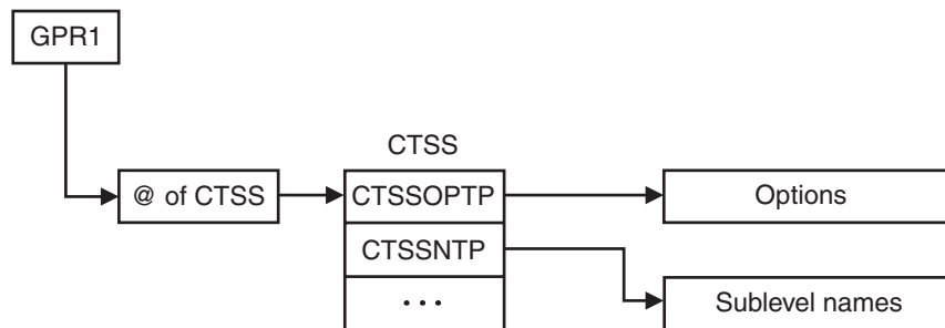
Figure 6-8. Information Passed to the Display Trace Exit Routine Through GPR 1
