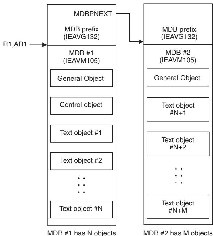
Figure 7-9. MDB Structure
