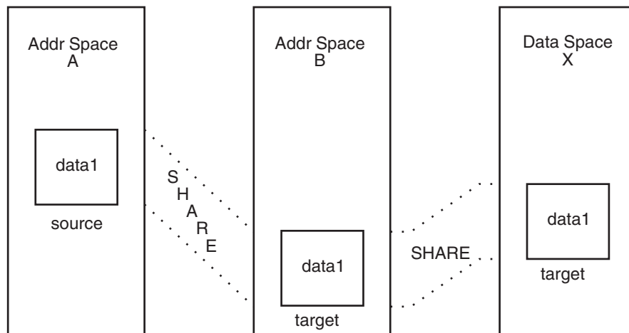
Figure 16-1. Data Sharing with IARVSERV
