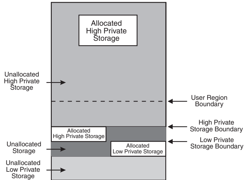
Figure 10-1. Low and High Private Storage Allocation
