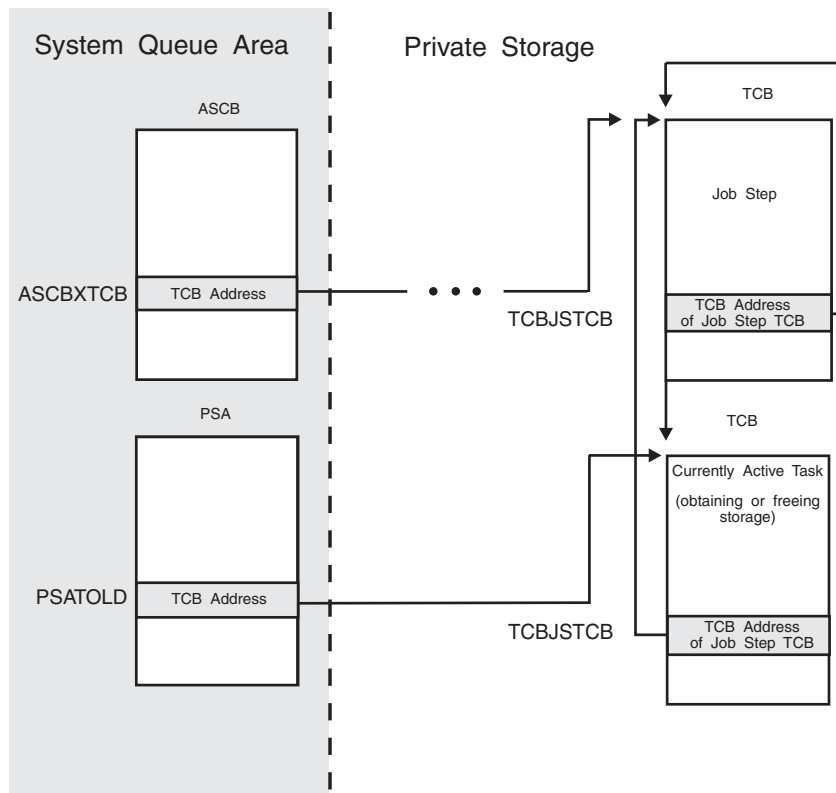
Figure 10-2. Task Structure Within an Address Space
