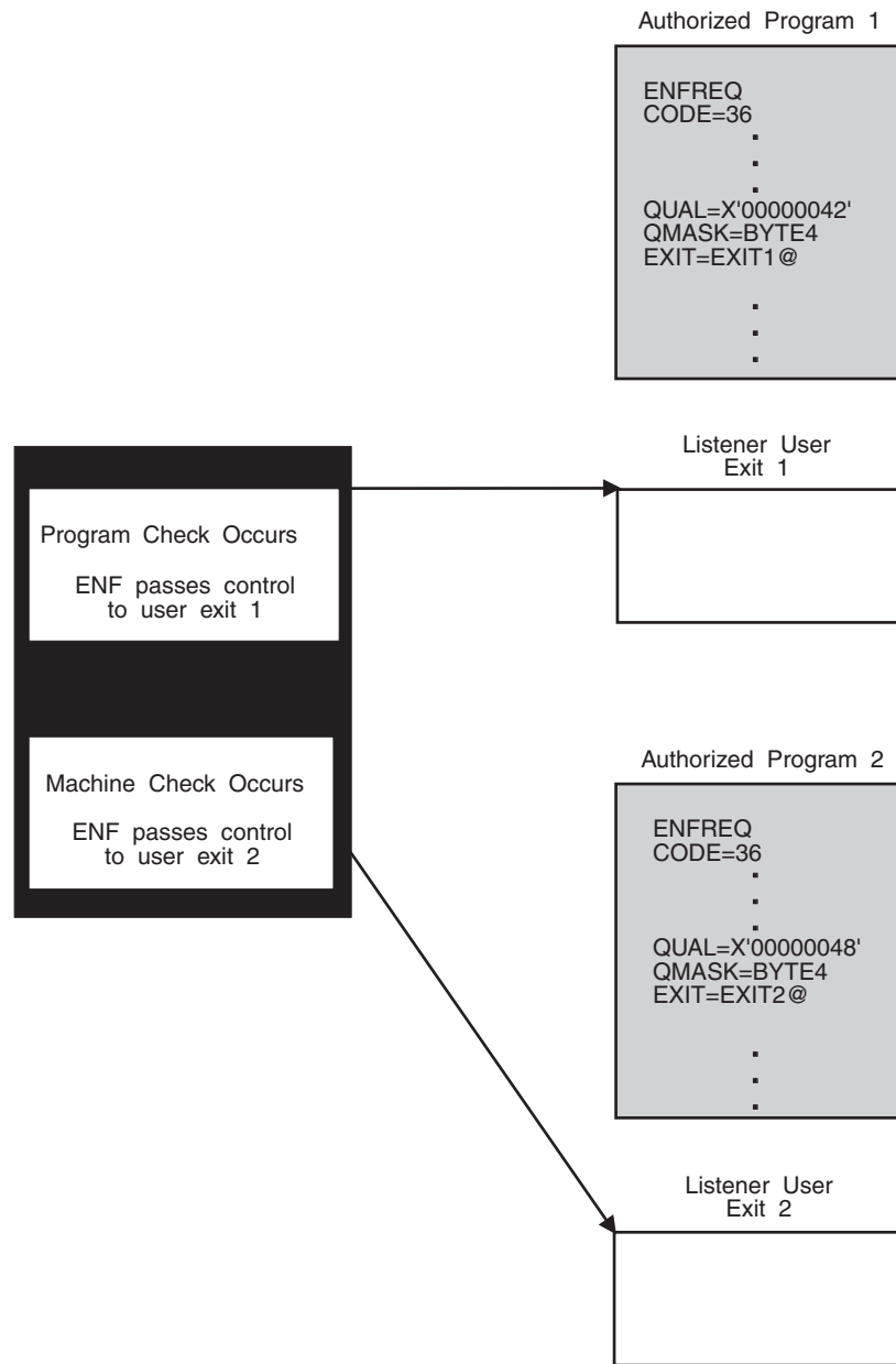
Figure 8-3. Authorized Programs with QUAL and QMASK
