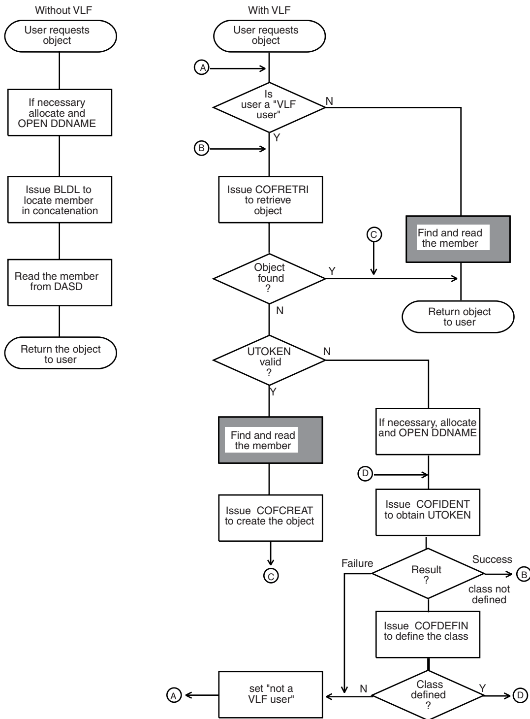
Figure 12-1. Retrieving an Object for an End User
