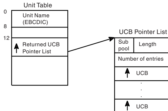
Figure A-7. Output from Function Code 3 (Return UCB Addresses)
