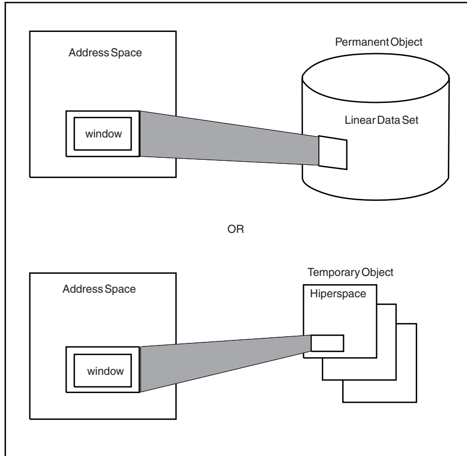
Figure 13-1. Mapping from an Address Space
