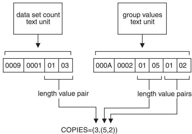
Figure 27-3. COPIES Keyword and its Dynamic Output Text Units
