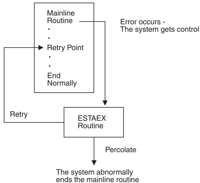
Figure 18-1. Mainline Routine with One Recovery Routine
