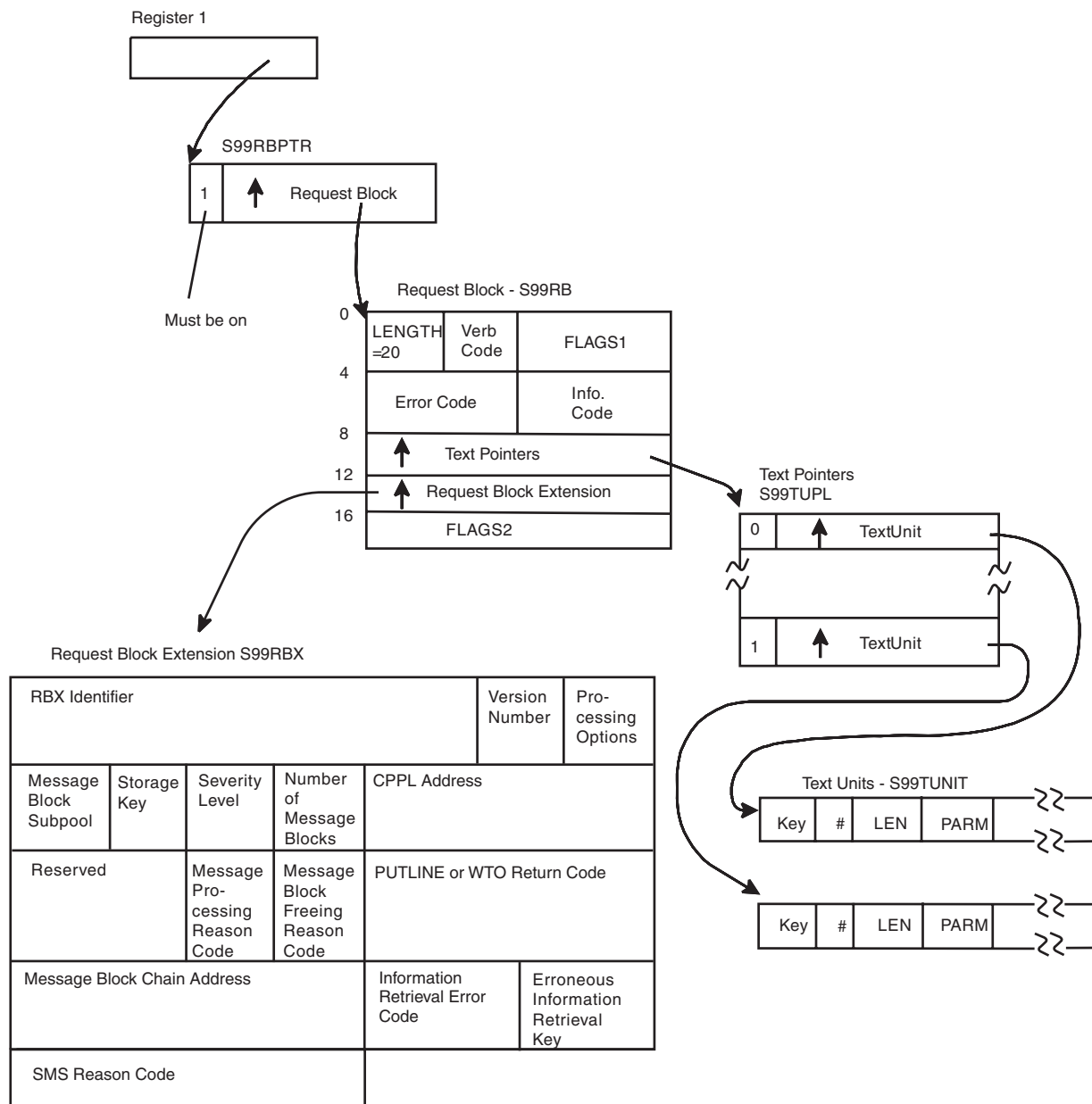
Figure 26-1. Structure of the SVC 99 Parameter List
