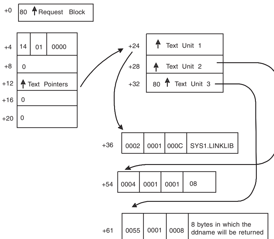
Figure 26-4. Parameter List Resulting from Dynamic Allocation Example
