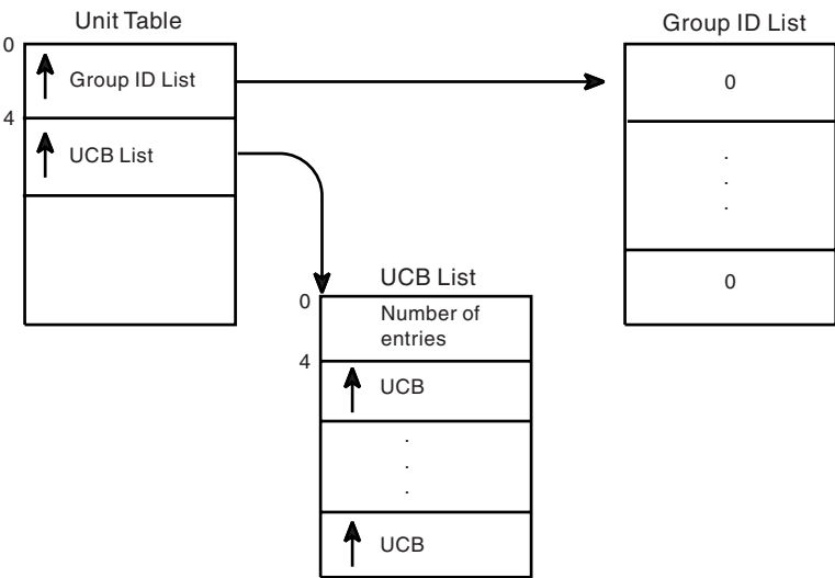
Figure A-8. Requesting Function Code 4 (Return Group ID)
