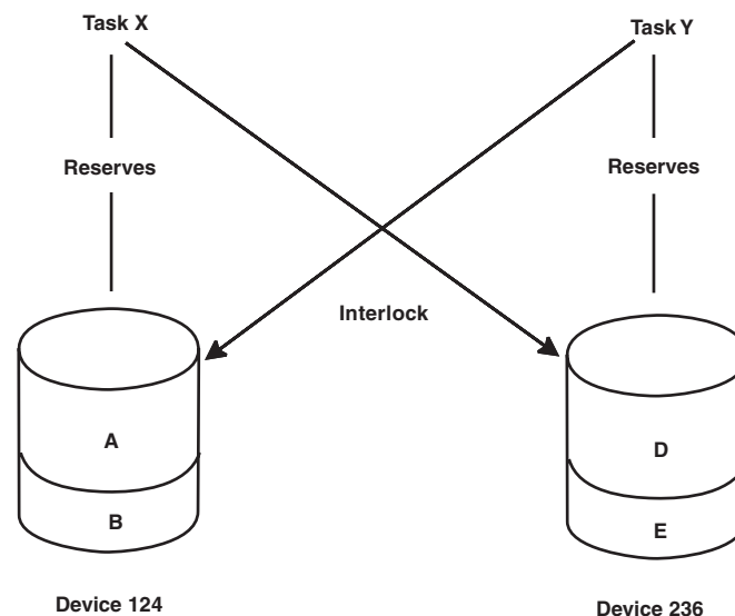
Figure 4-1. Example of an Interlock Environment
