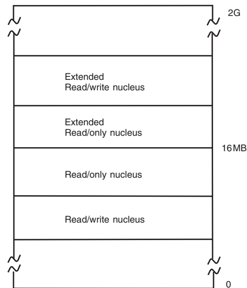
Figure 17-1. Virtual Storage Map of DAT-ON Nucleus
