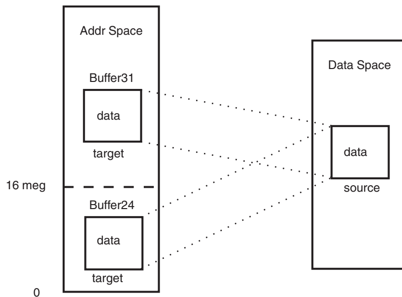
Figure 16-2. Sharing Storage with IARVSERV
