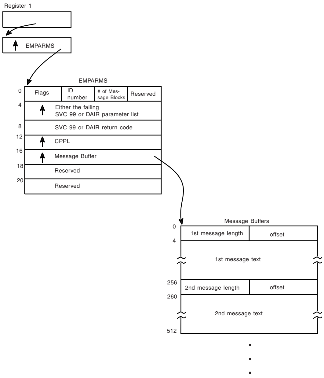
Figure 26-2. Structure of Input Parameter List to IEFDB476
