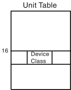
Figure A-17. Requesting Function Code 11 (Return Unit Names for a Device Class)
