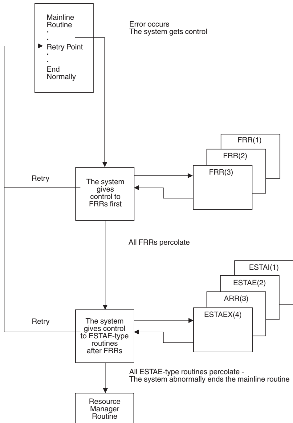
Figure 18-2. Mainline Routine with Several Recovery Routines
