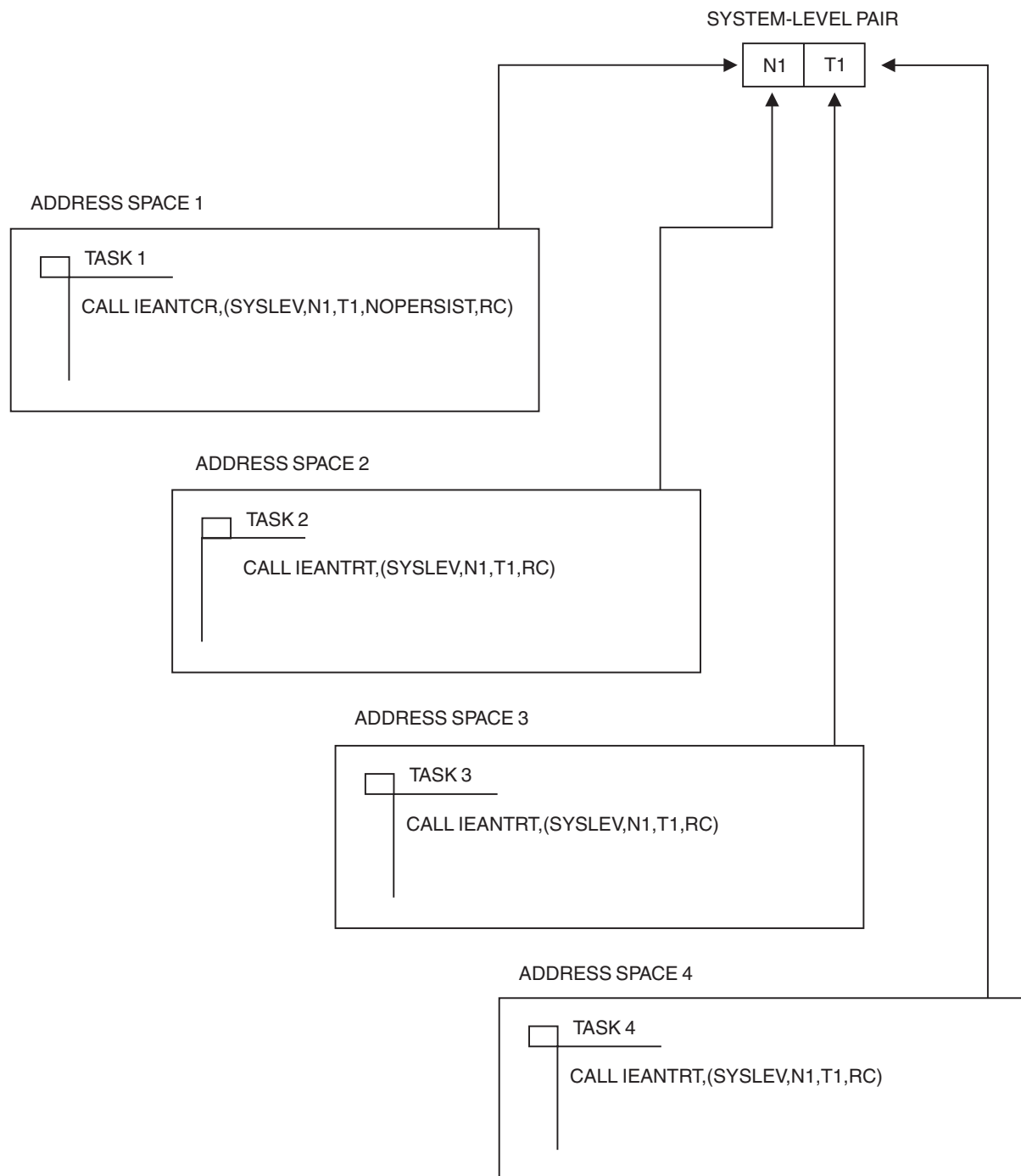
Figure 14-2. Using the System Level in a Multiple Address Space Environment
