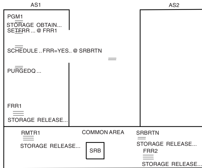
Figure 9-1. Example of Scheduling an SRB
