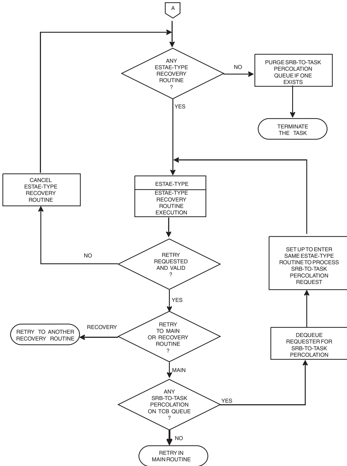
Figure 18-5. Routing Control to Recovery Routines (Part 2 of 3)
