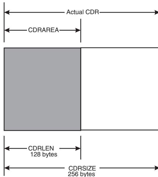
Figure 24-2. Comparison of CDRLEN to CDRSIZE
