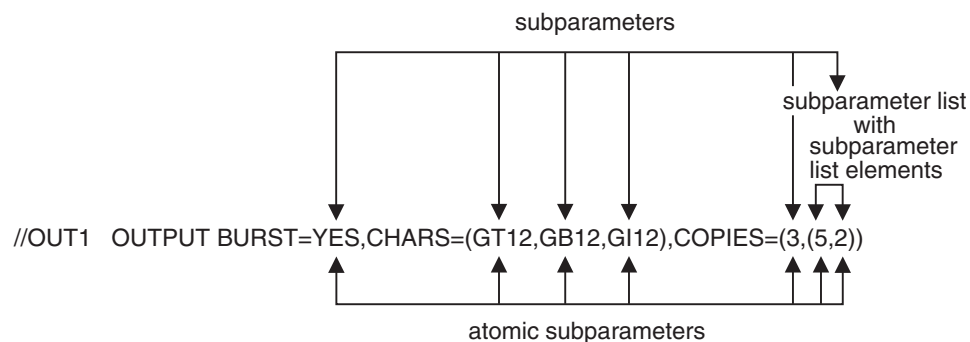
Figure 27-2. Sample OUTPUT JCL Statement
