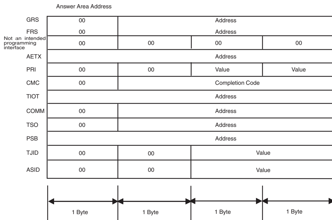
Figure 2-3. EXTRACT Answer Area Fields
