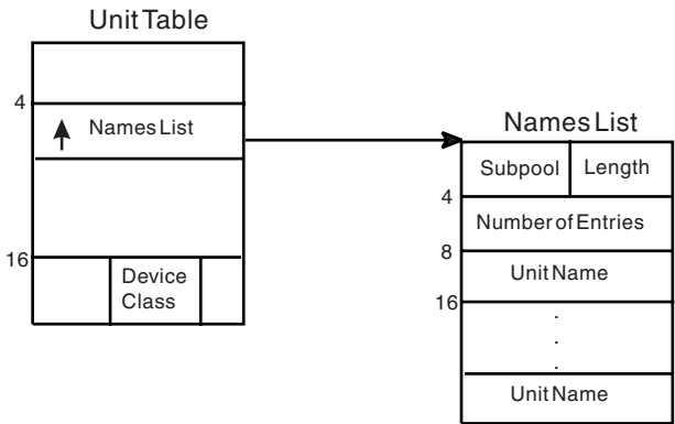
Figure A-18. Output from Function Code 11 (Return Unit Names for a Device Class)
