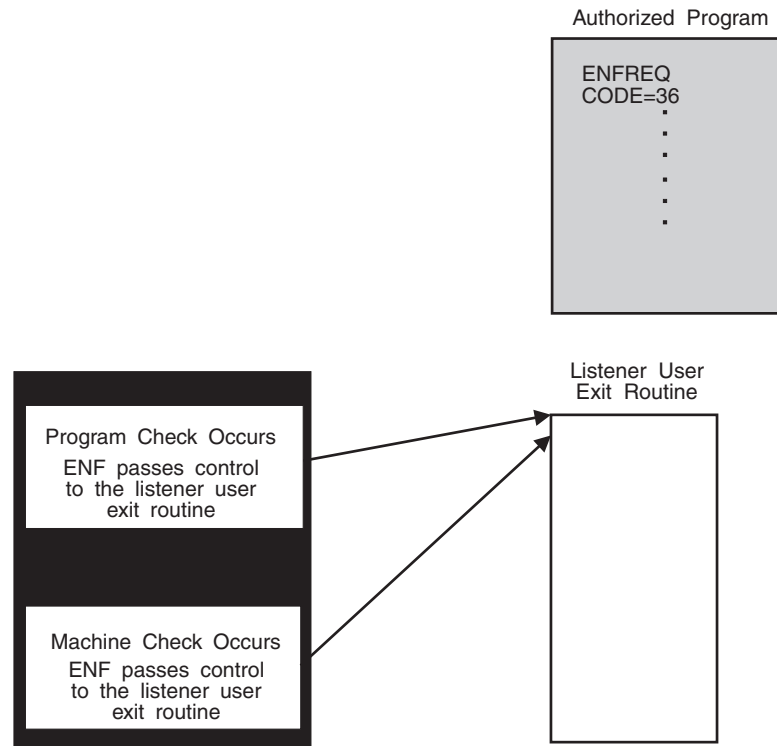
Figure 8-1. Authorized Program without QUAL and QMASK
