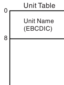
Figure A-6. Requesting Function Code 3 (Return UCB Addresses)
