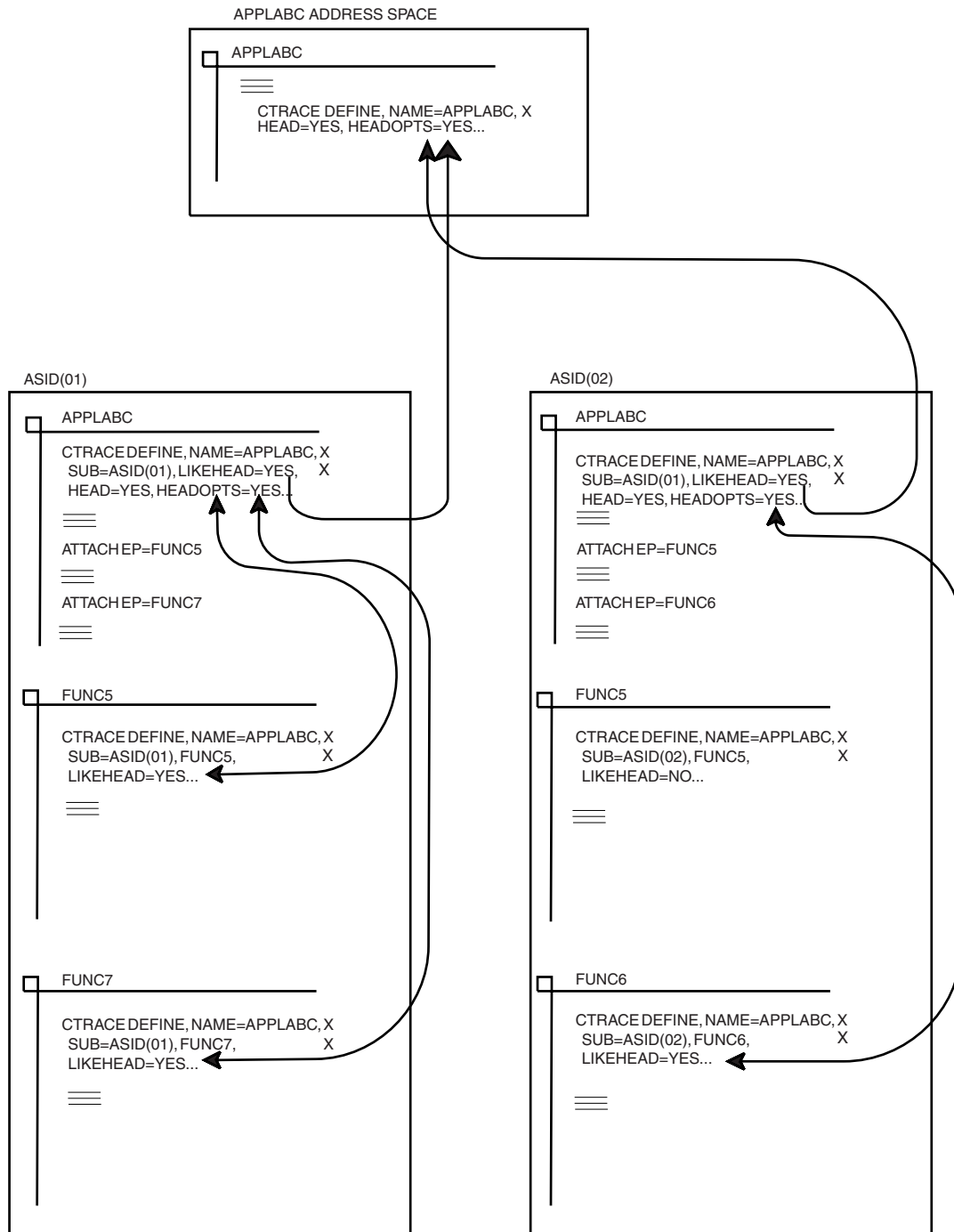
Figure 6-4. Setting up Multiple Traces with CTRACE DEFINE
