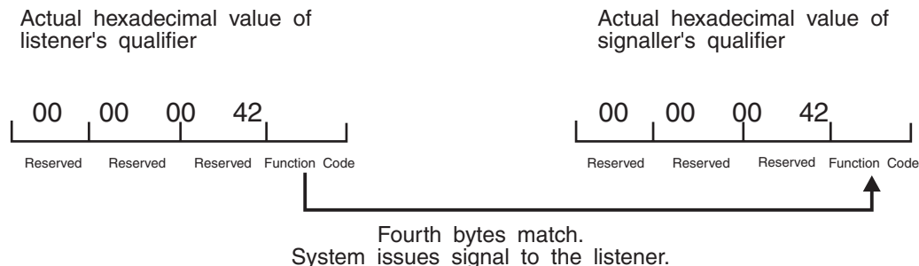
Figure 8-2. Qualifier for a Program Check
