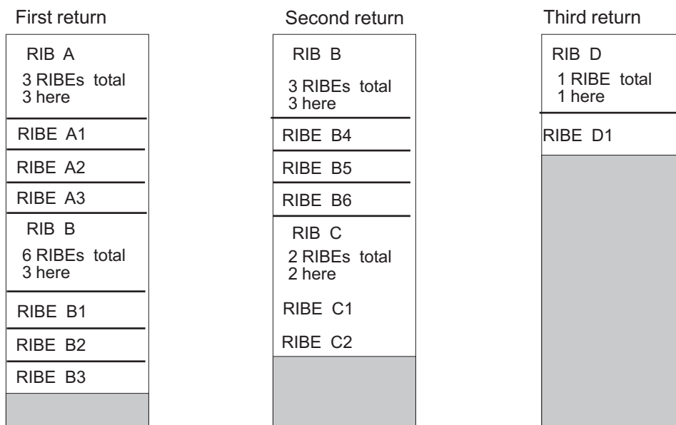
Figure 5-2. Work Area Contents for GQSCAN with a Scope of LOCAL or GLOBAL
