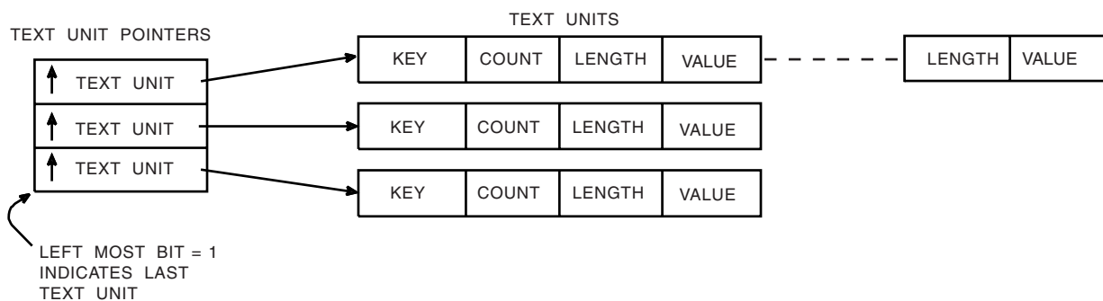
Figure 27-1. Text Units and Text Unit Pointers
