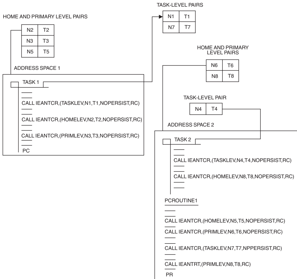
Figure 14-1. Using the Primary Level in a Cross-Memory Environment
