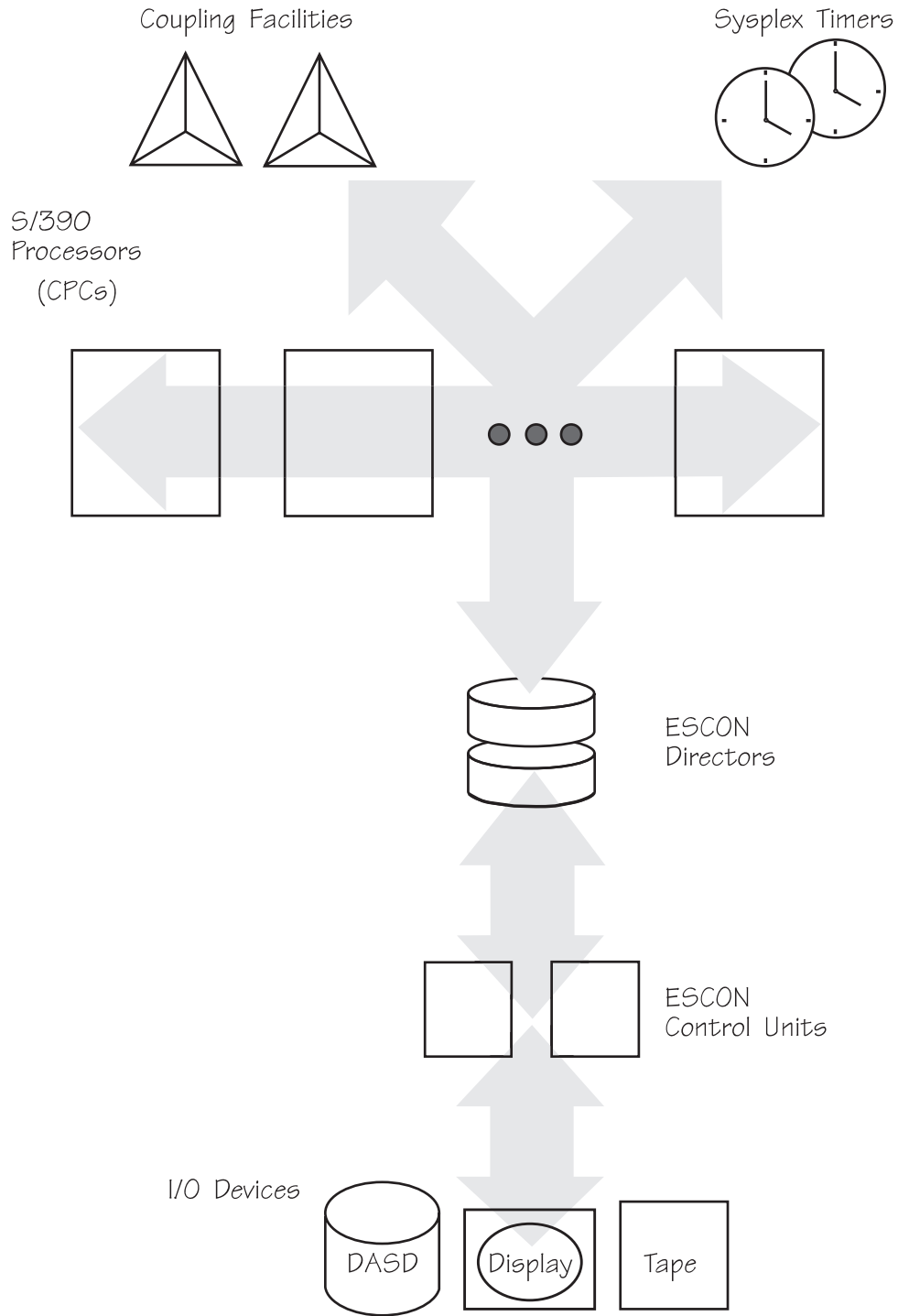
Figure 2. Sysplex Structure
