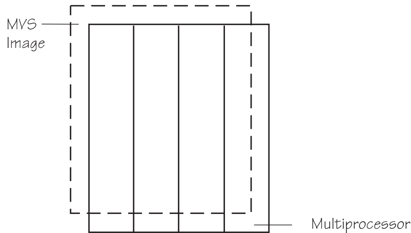
Figure 4. A Tightly Coupled Multiprocessor
