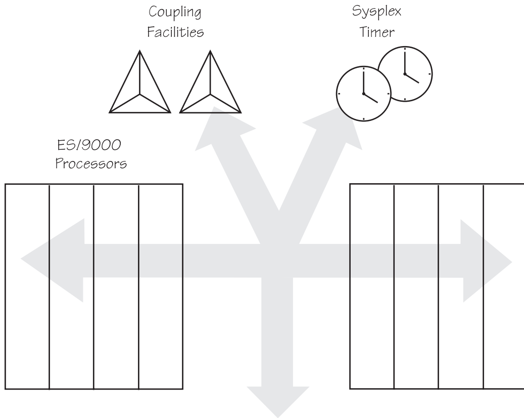
Figure 20. Large Systems Sysplex Configuration
